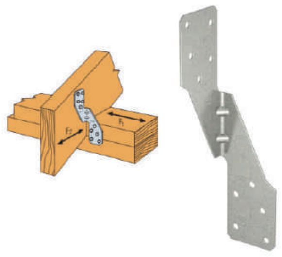
FIGURE 3-27 - SOURCE: SIMPSON STRONG-TIE
