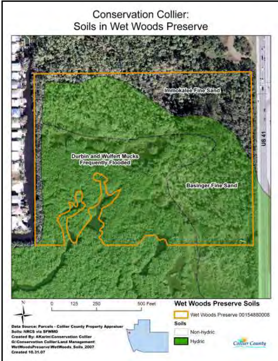
Figure 5: Soil Units at the Wet Woods Preserve
