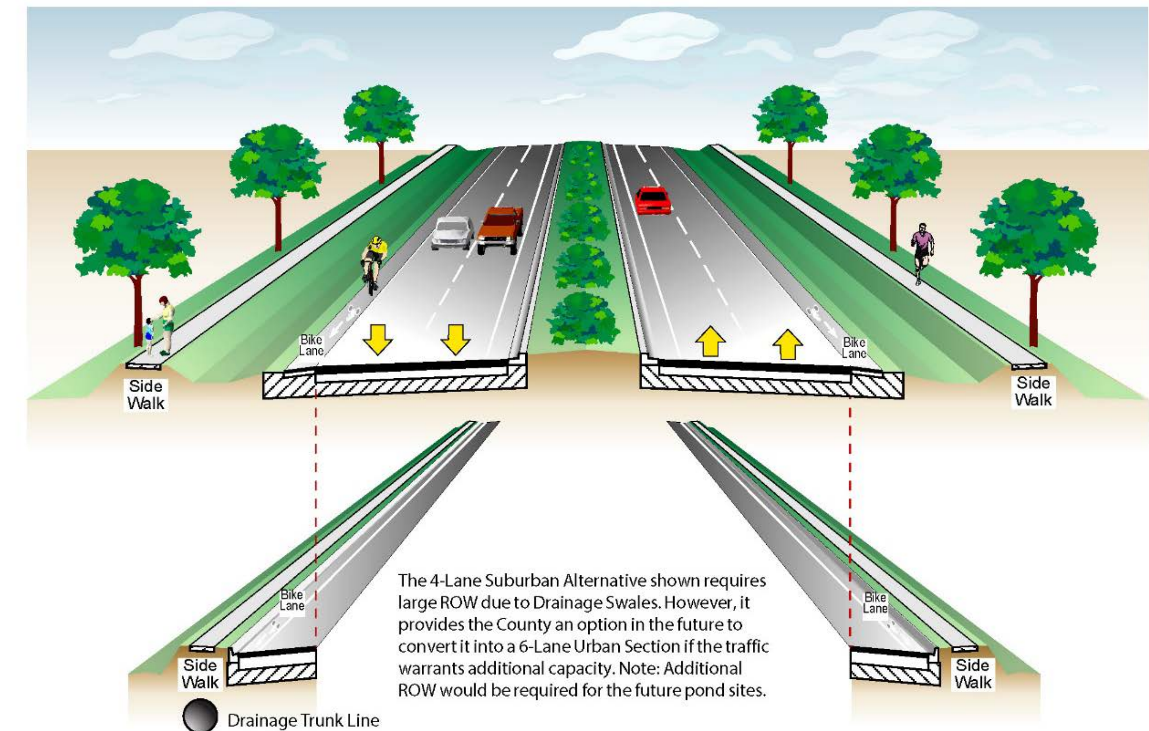
Proposed 4-Lane Suburban Typical Section with Drainage Swales
