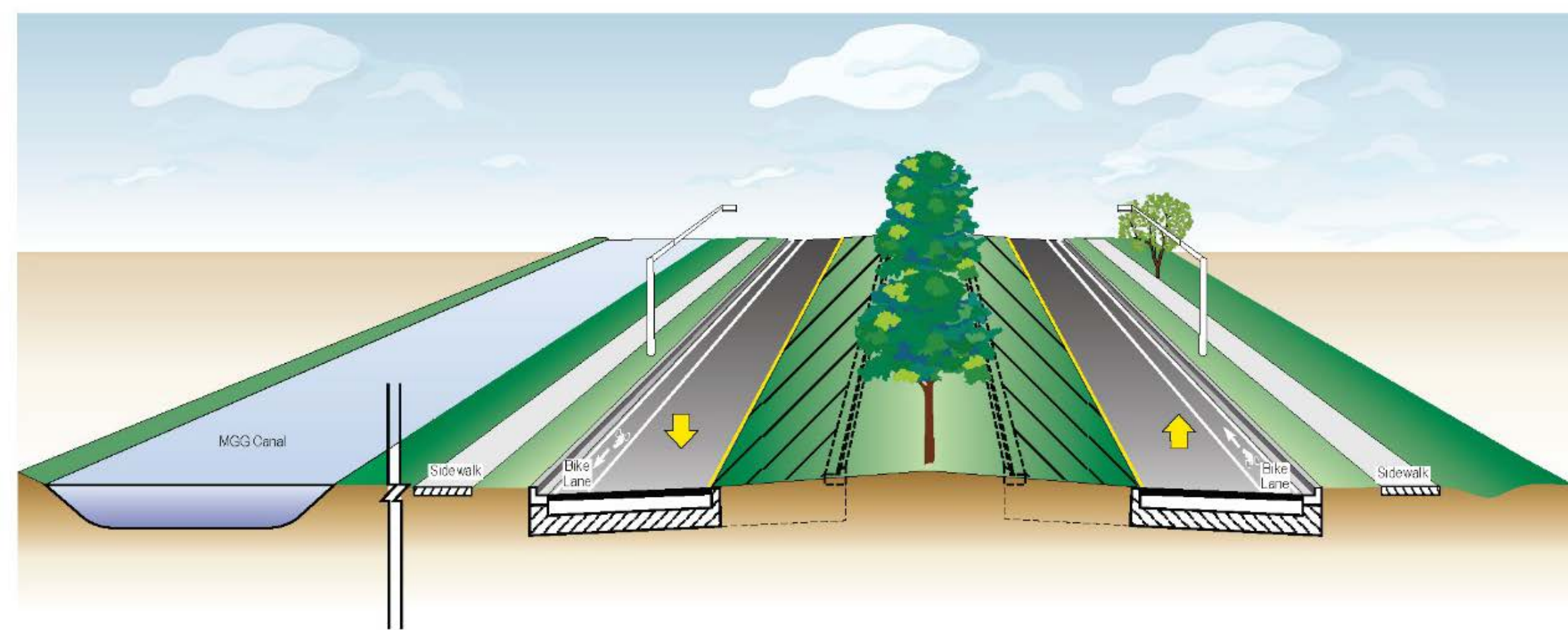
Proposed 2-Lane Urban Typical Section with Provisions for Median Expansion to 4-Lanes "S" Connector Alternative (Adjacent to MGG Canal)
