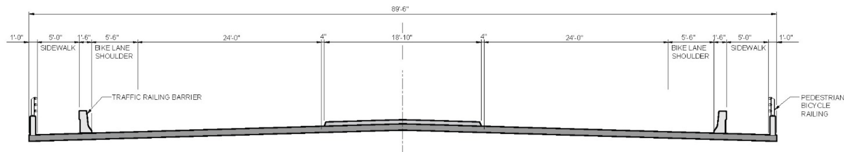
Proposed 4-Lane Bridge Typical Section Roadway typical section evaluation will determine bridge configuration - Randal Blvd Over Main Golden Gate Canal Alternative - Randal Blvd Over Faka Union Canal Alternative
