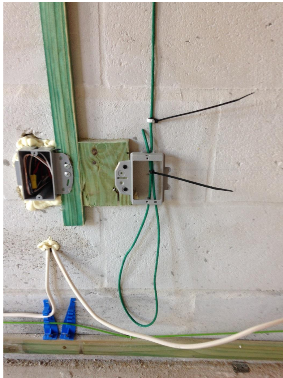
510- Primary alarm system work performed, before insulation and drywall is installed
