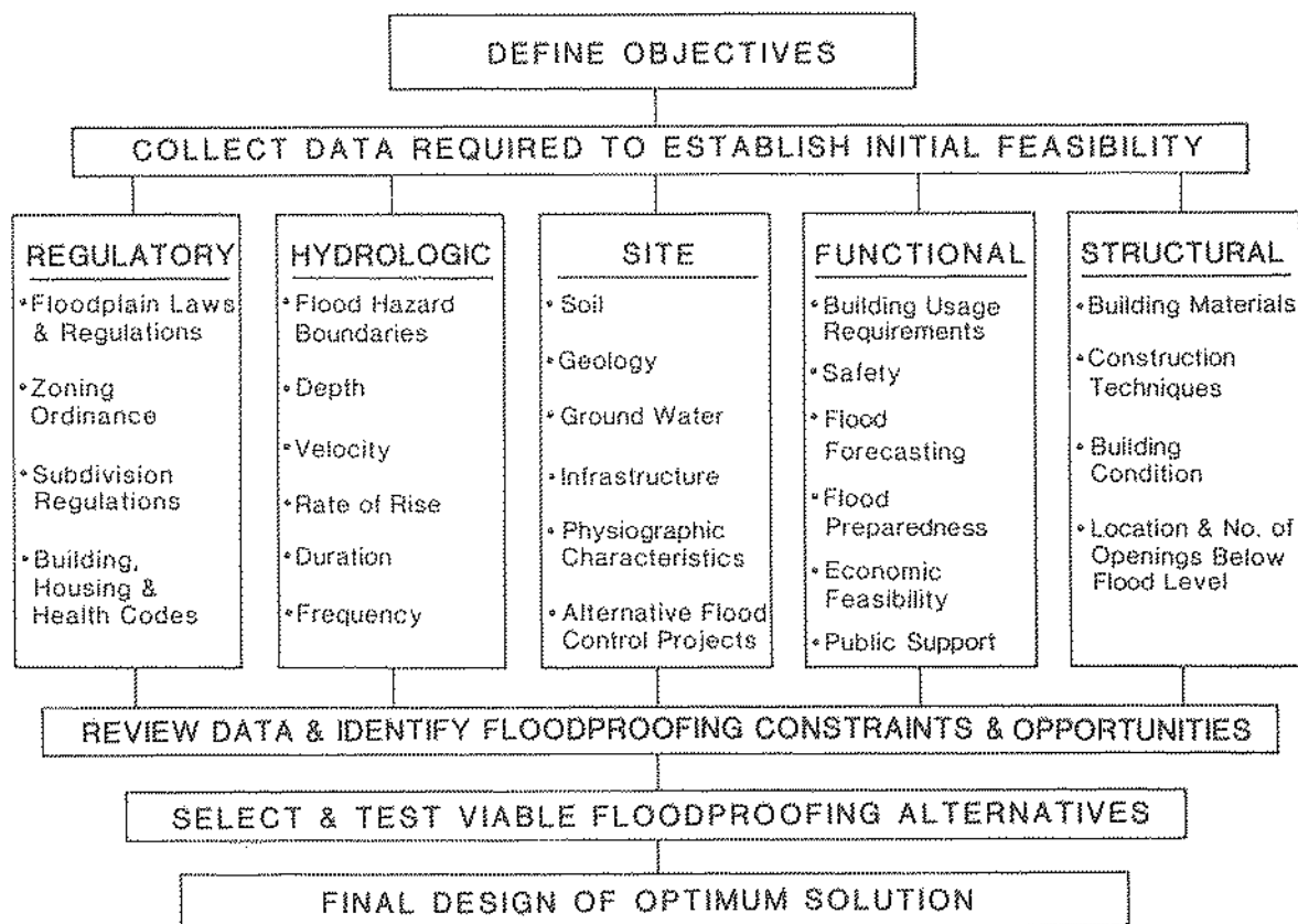
Figure 11-1. General Floodproofing Design Process
