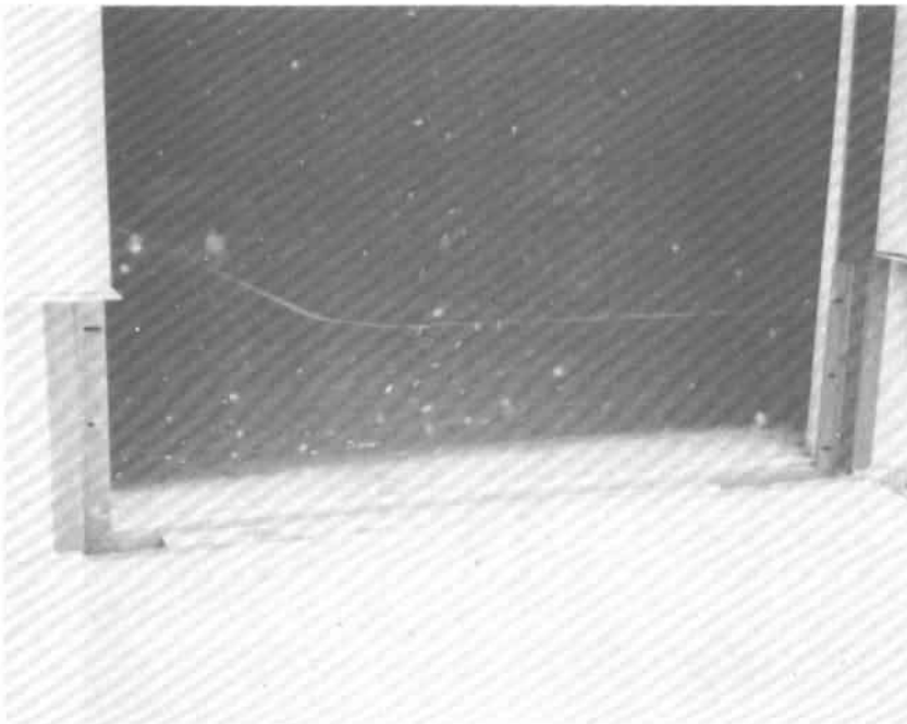
Frame for mounting flood shield on loading dock door. A 4" x 4" piece of timber is used to facilitate traffic over a slot designed to receive and seal the flood shield.
