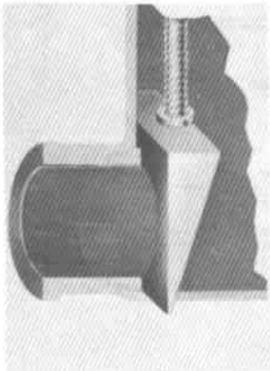
SHEAR-GATE VALVE
