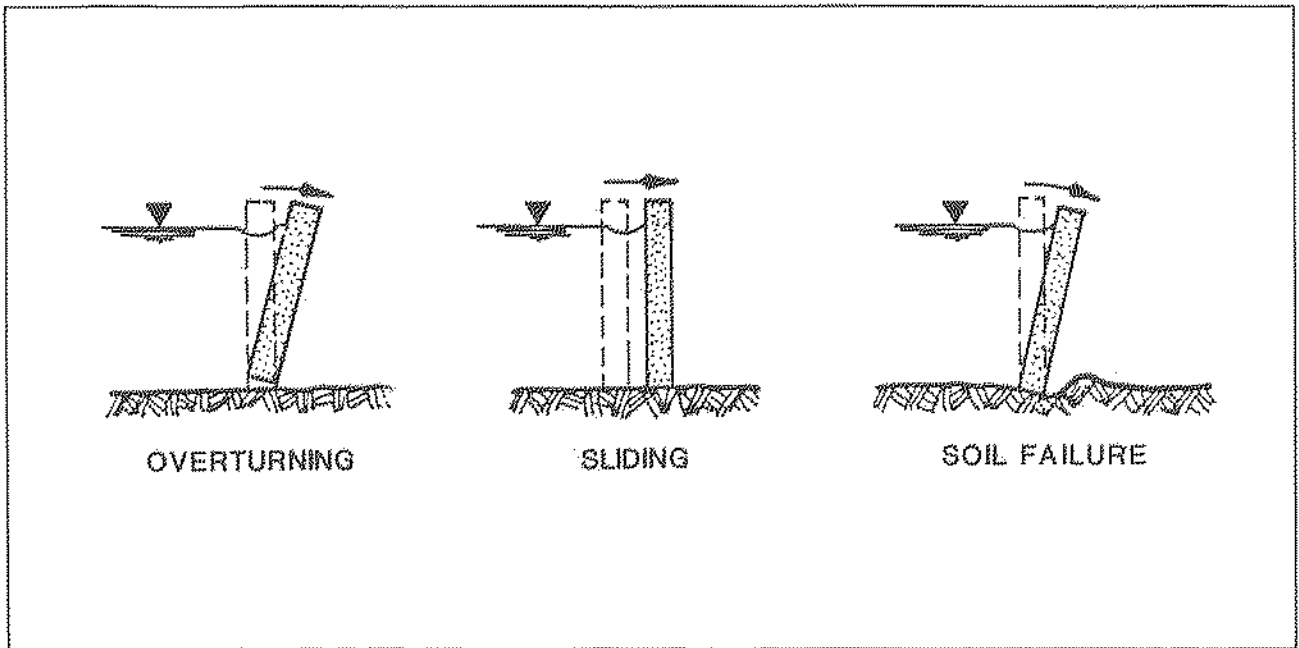
Figure III-48. Floodwall Stability
