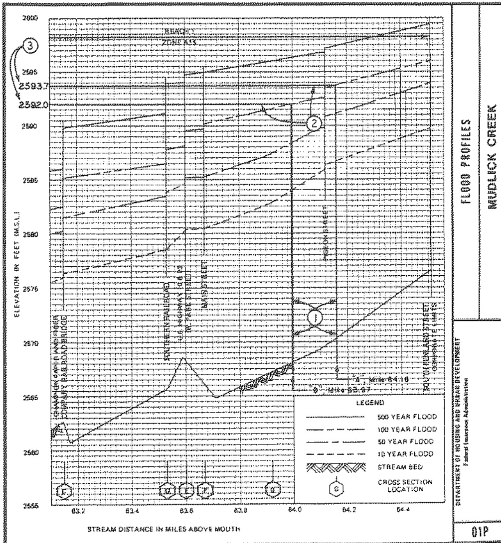
FIGURE F-2 EXAMPLE FLOOD PROFILE Circled numbers correspond to steps listed for determining applicable flood elevations.
