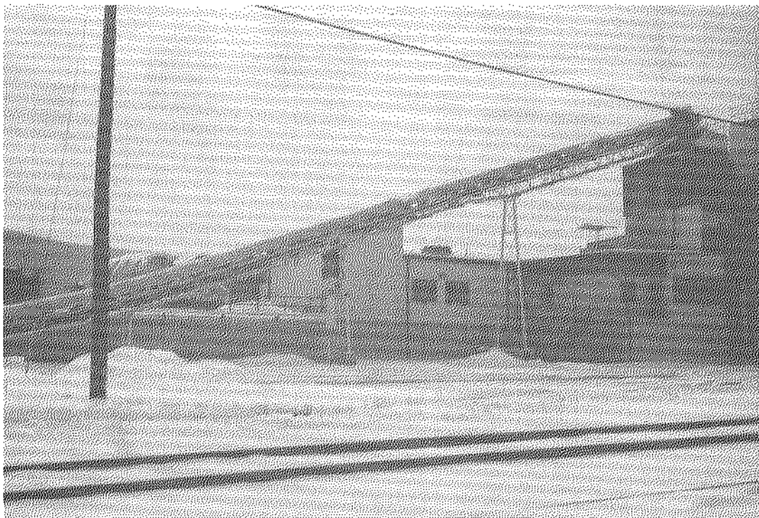
Control building is elevated on earth fill that is enclosed by concrete retaining walls. This technique minimizes space requirements because areas for slope transition are not required.
