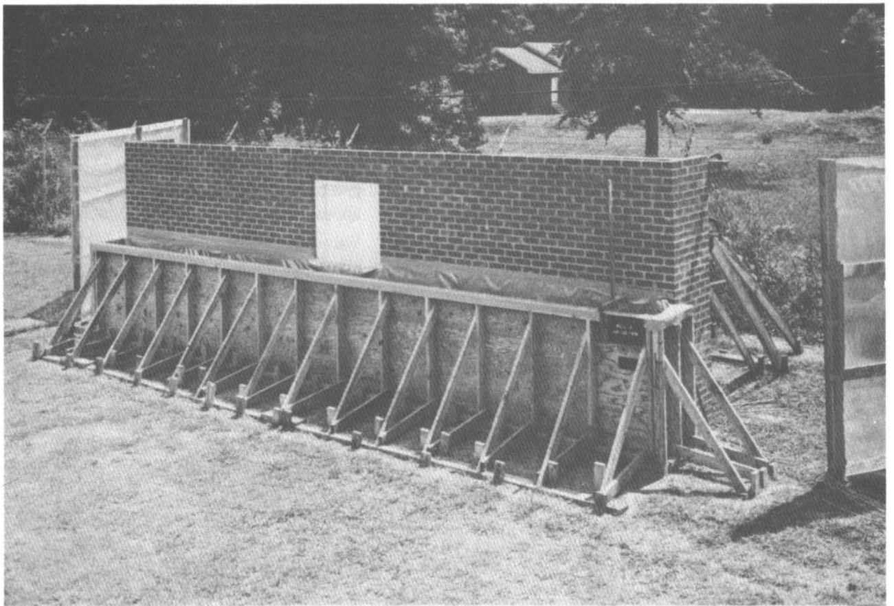
Figure III-38. Testing Bin
