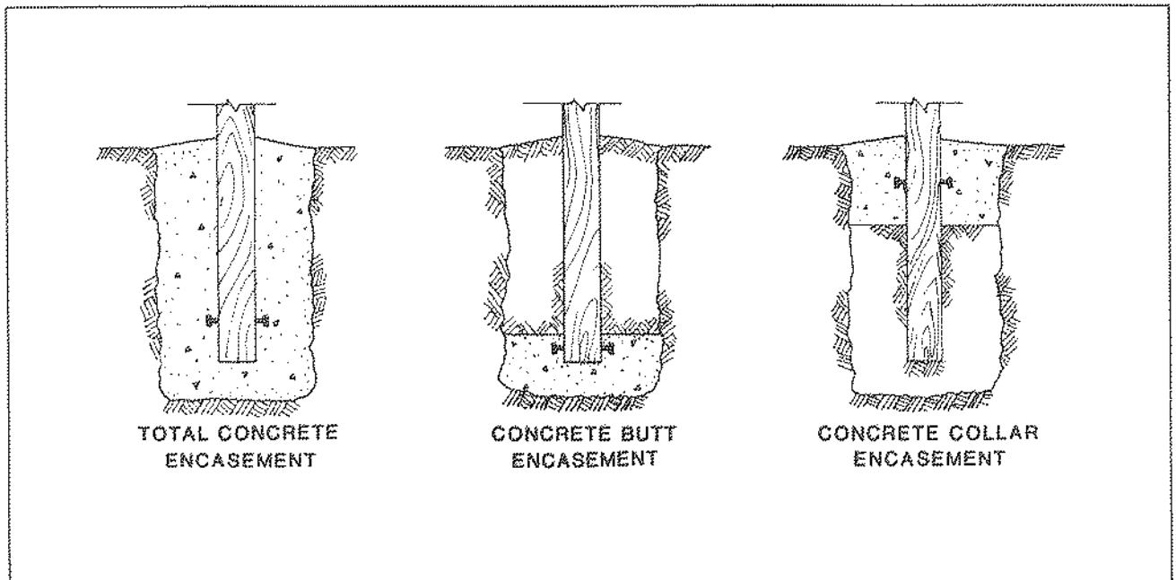
Figure III-1. Concrete Backfill
