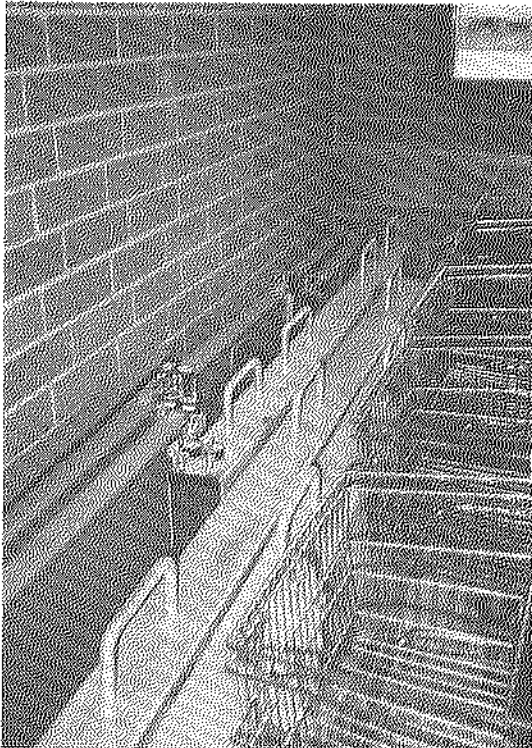
Stored flood shields (Note pneumatic seal valves).
