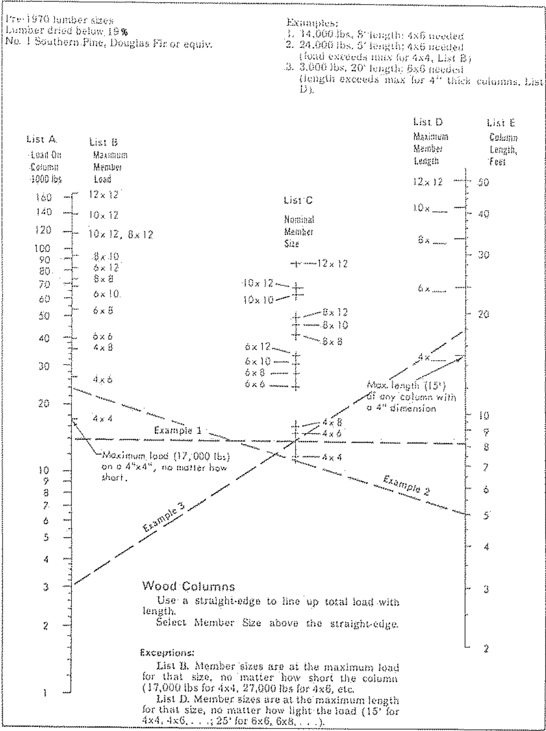
Figure III-6. Approximate Loads on Wood Posts
