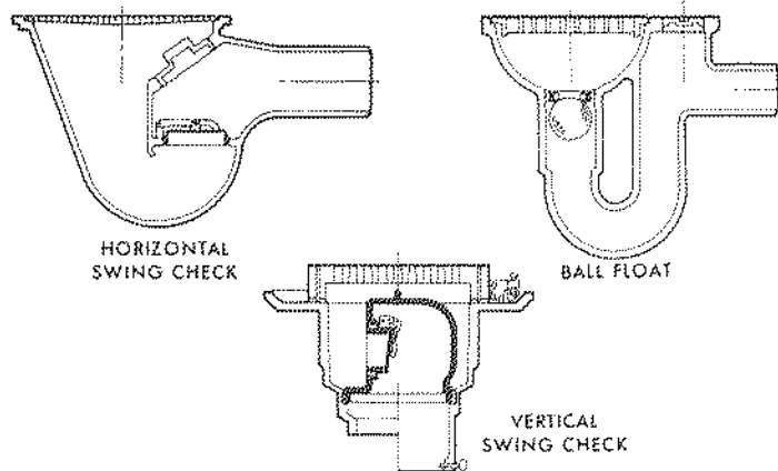
VARIOUS EXAMPLES OF BACKWATER VALVES
