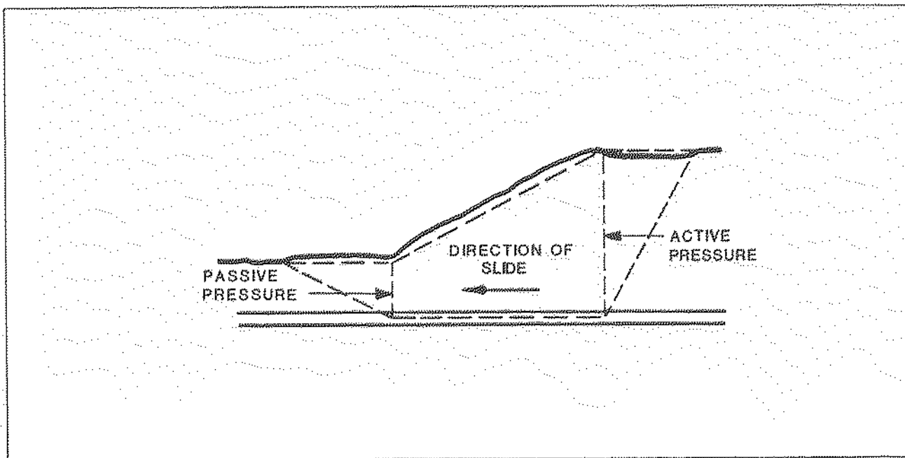
Figure III-54. Translatory Slide
