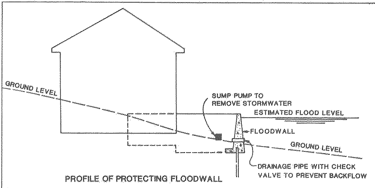
Figure I-6. Flood Protection With Low Floodwall
