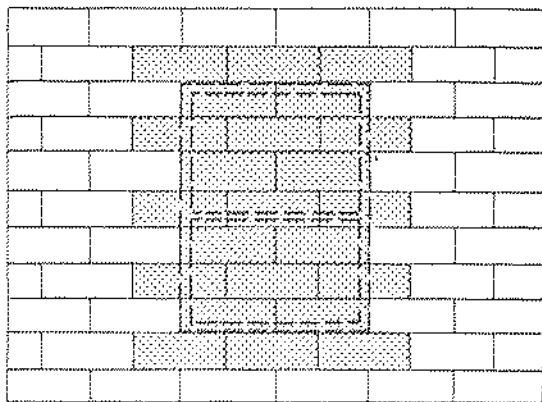
Figure I-1. Permanent Window Closure in existing masonry wall.
