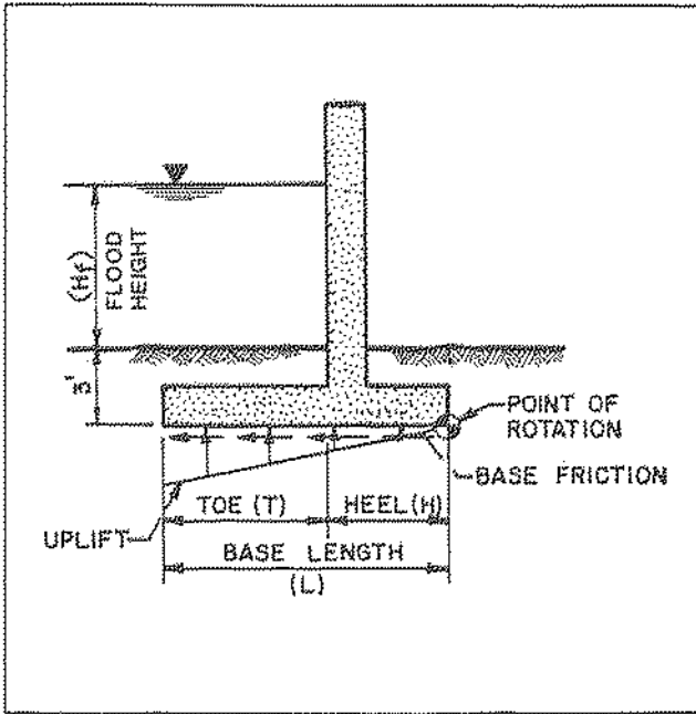
Figure III-50. Stability-Cantilever Floodwalls
