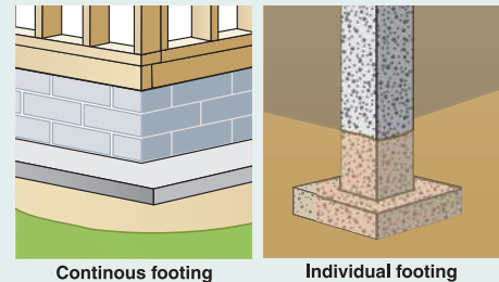
Continuous footing
