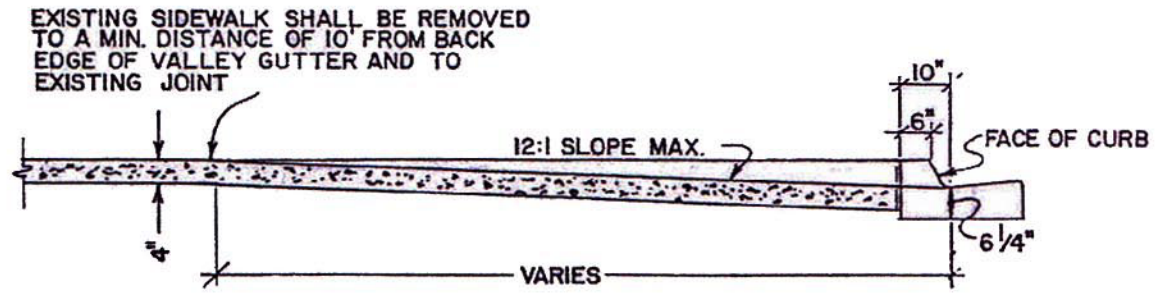
SECTION AA
