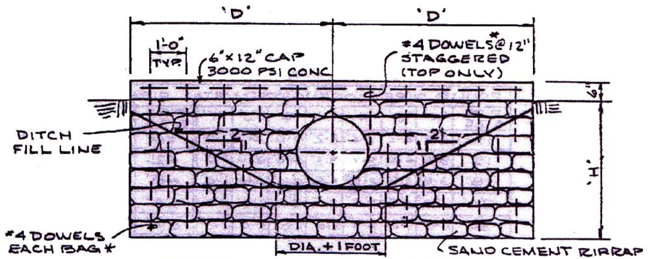
FRONT ELEVATION-SINGLE PIPE
