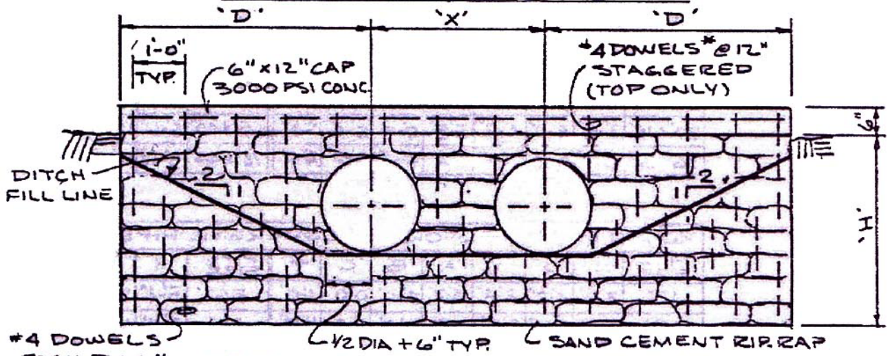
FRONT ELEVATION-MULTIPLE PIPE
