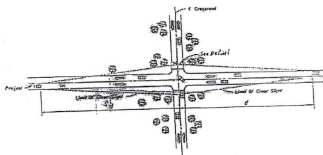
2 LANE UNDIVIDED • SIGNALIZED OR STOP SIGN CONTROLLED
