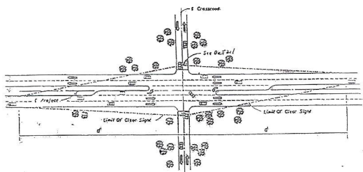
MULTILANE DIVIDED • SIGNALIZED OR STOP SIGN CONTROLLED
