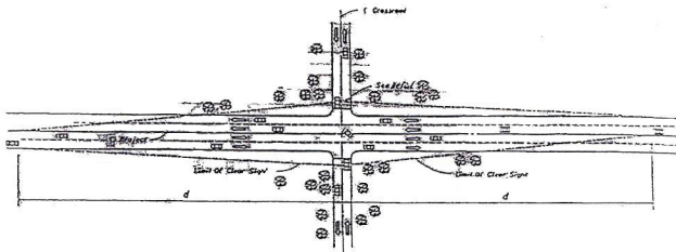
MULTILANE UNDIVIDED • SIGNALIZED OR STOP SIGN CONTROLLED
