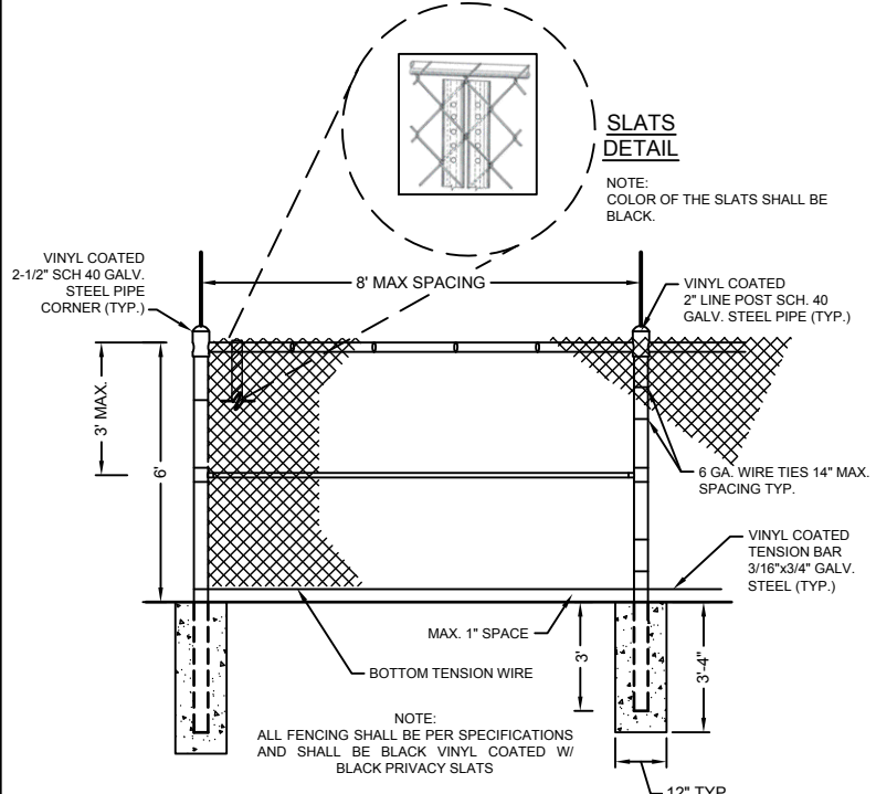
CHAIN LINK FENCE DETAIL
