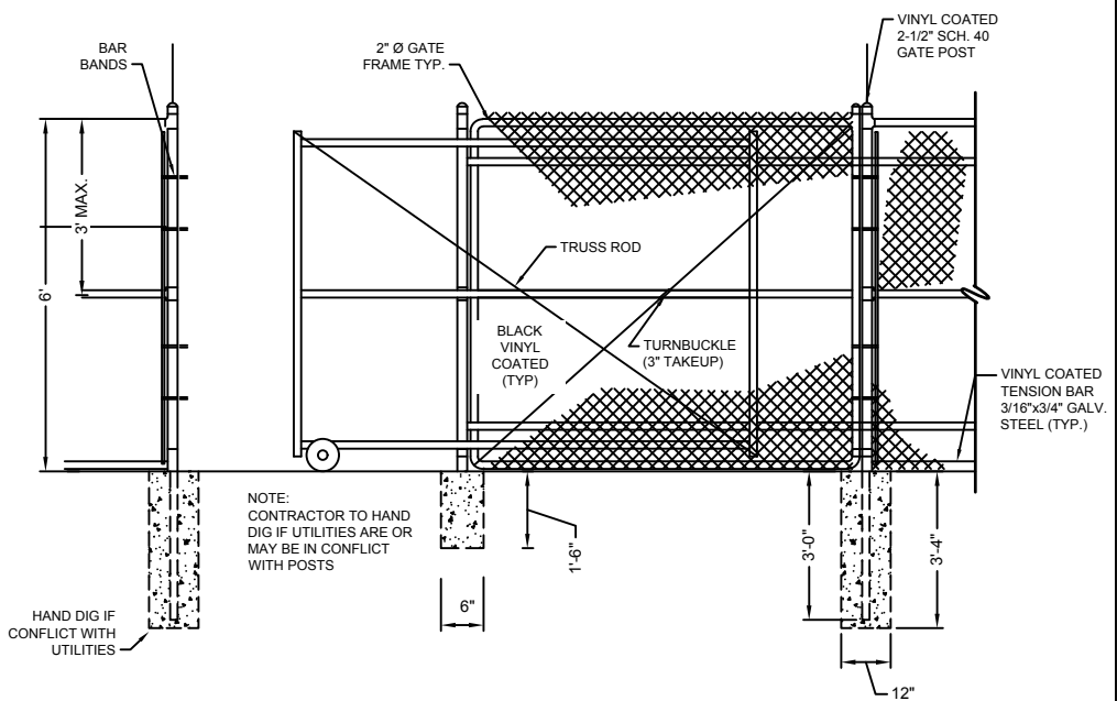
CHAIN LINK FENCE GATE DETAIL
