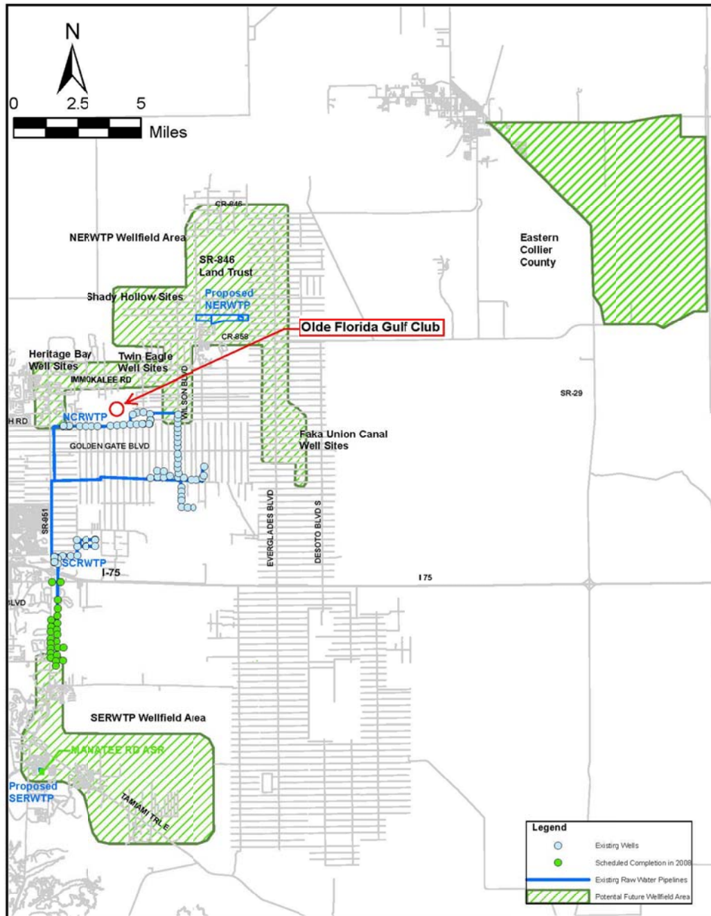
Figure 7-7 2008 Water Master Plan Update Potential Future Wellfield Areas
