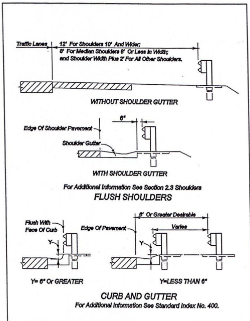
Figure 2.11.1 Clearance to Guardrail
