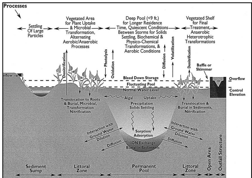
▲ Figure 1. Idealized Wet Detention Pond
