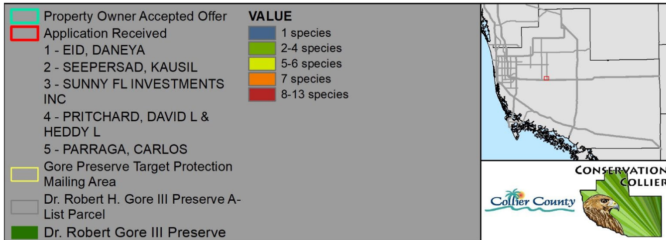
Figure 12 - CLIP4 Potential Habitat Richness
