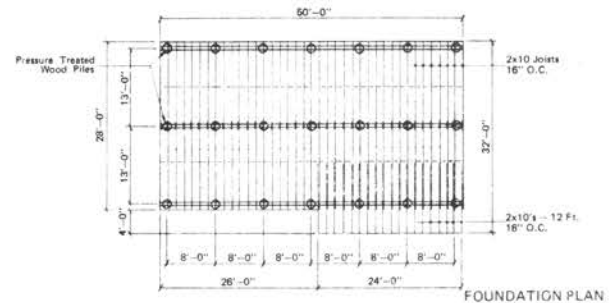
FOUNDATION PLAN
