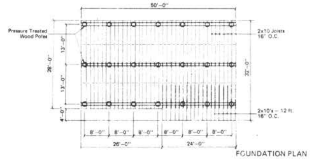
FOUNDATION PLAN
