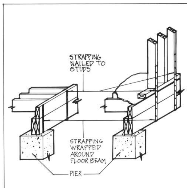
Figure 4.43. Metal Strapping
