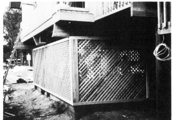
Figure 4.54. Breakaway Walls
